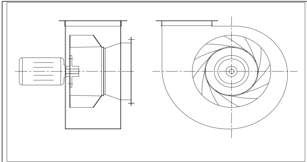
FLANGE MOUNTED BLOWER
