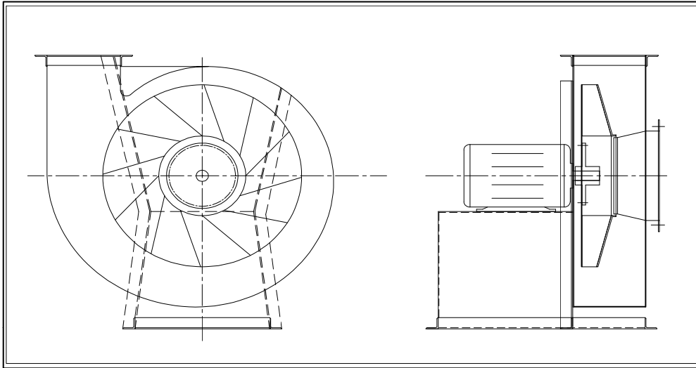
FOOT MOUNTED BLOWER
